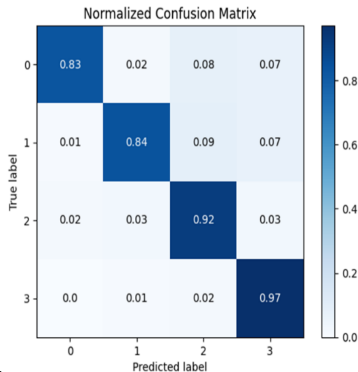
Fig. 1 - Decision tree normalized confusion matrix.
