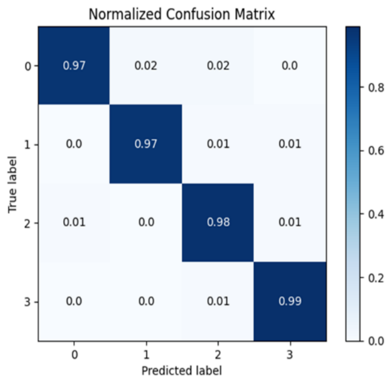
Fig. 2 - Random forest normalized confusion matrix.
